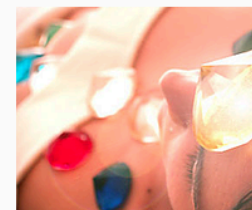
Crystals
